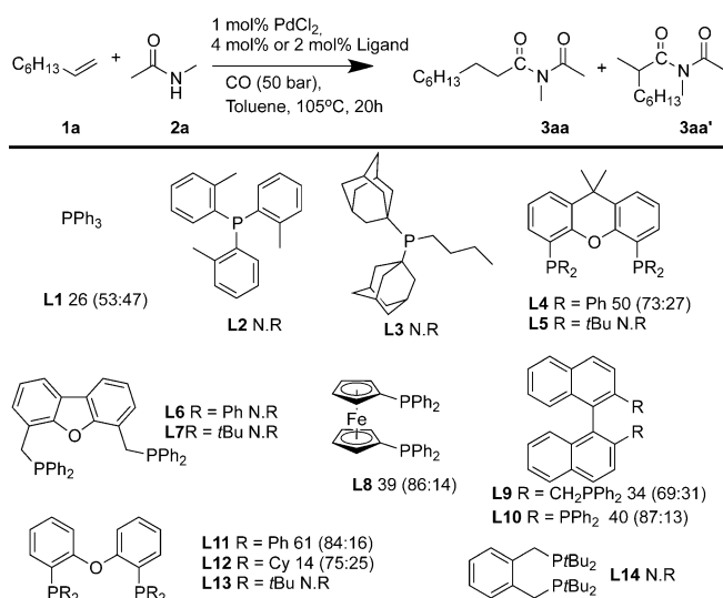
Scheme 2. Hydroamidocarbonylation of 1-octene. Reaction conditions: Ligand variation. 2a (1.0 mmol), 1a (1.0 mmol), \text{PdCl}_2 (1 mol%), monodentate ligand (4 mol%) or bidentate ligand (2 mol%), toluene (2 mL), CO (50 bar) heating at 105°C for 20 h. Yield (%) of the mixture of 3aa and 3aa' determined by GC using isooctane as an internal standard, the number in parenthesis indicates the 3/3' selectivity determined by GC. N.R. indicates no observable product by GC.
